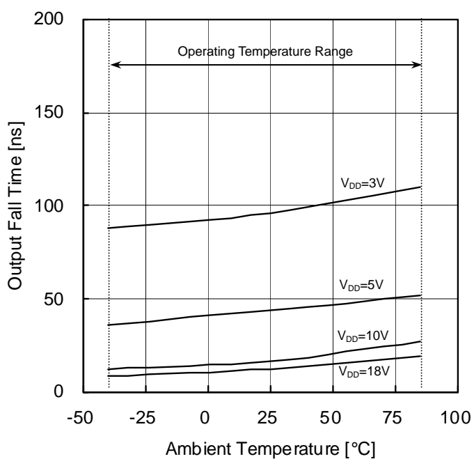
Figure 7. Output falling time t_{THL}
